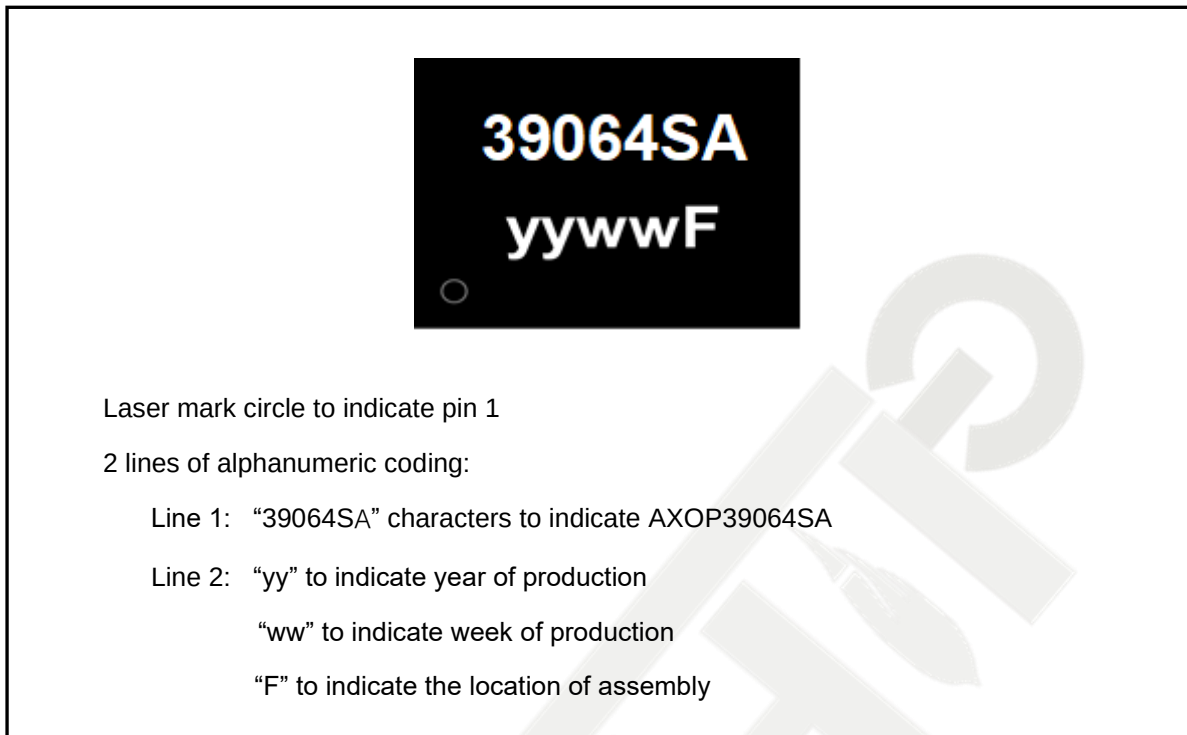
Figure 30 QFN16 Marking Information
