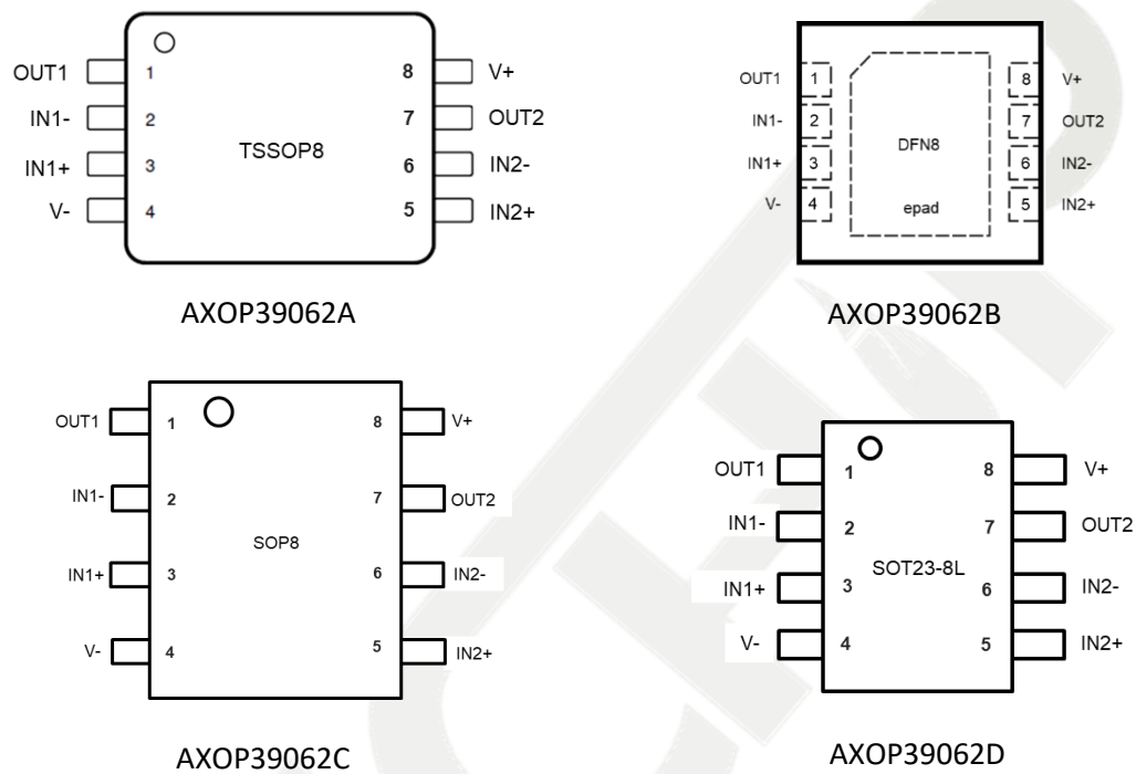
Figure 3 AXOP39062A/B/C/D Pinouts
