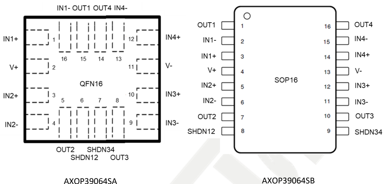
Figure 6 AXOP39064SA/B Pinouts
