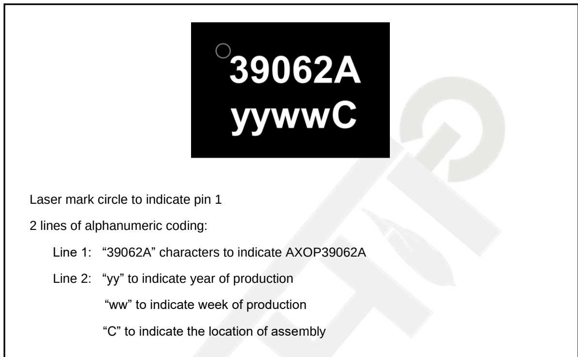
Figure 25 TSSOP8 Marking Information
