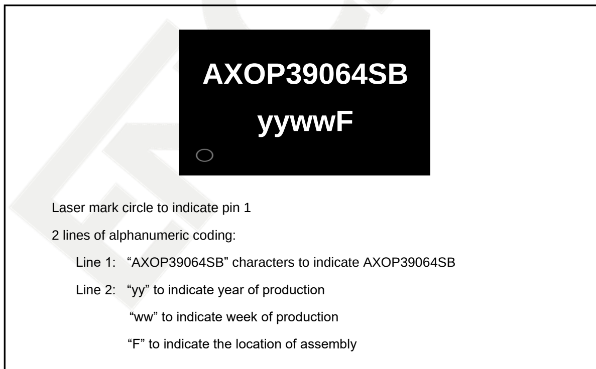
Figure 31 SOP16 Marking Information
