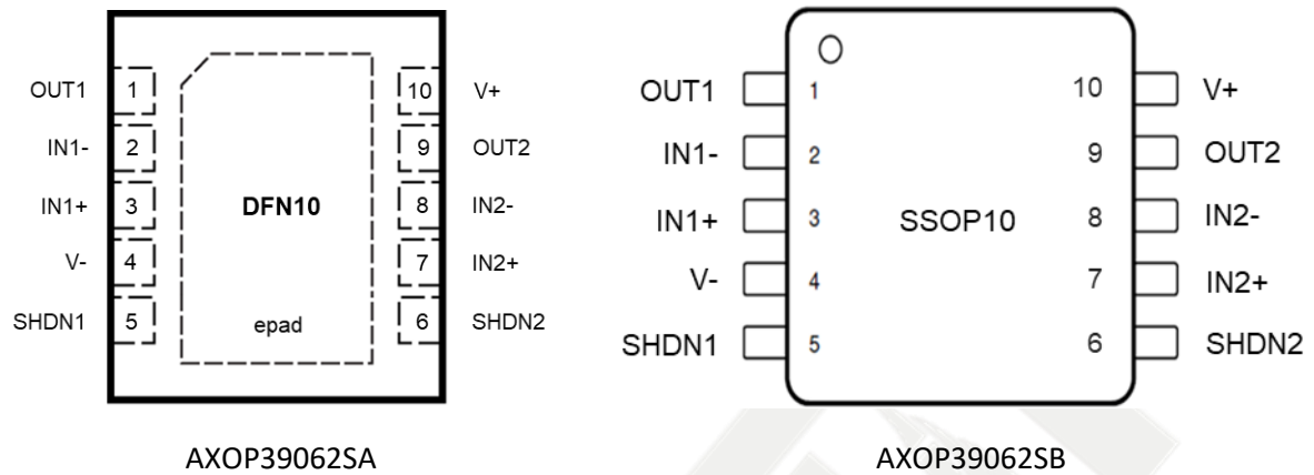
Figure 4 AXOP39062SA/B Pinouts
